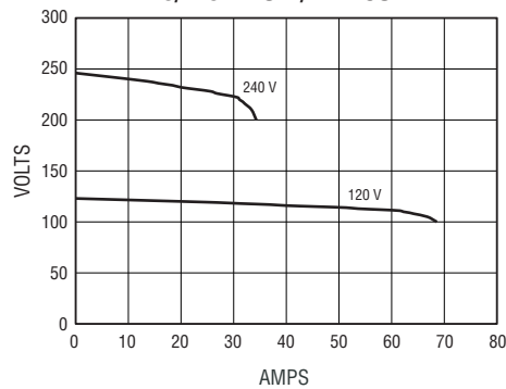
120/240 V VOLT/AMP CURVE
